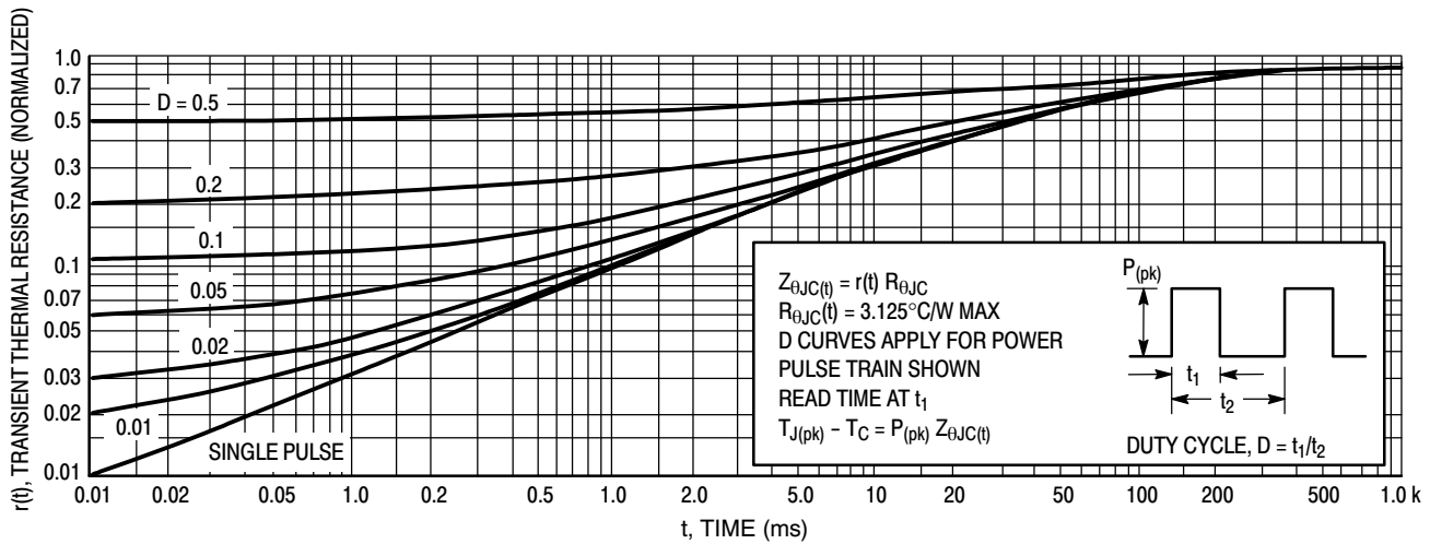
Figure 4. Thermal Response
